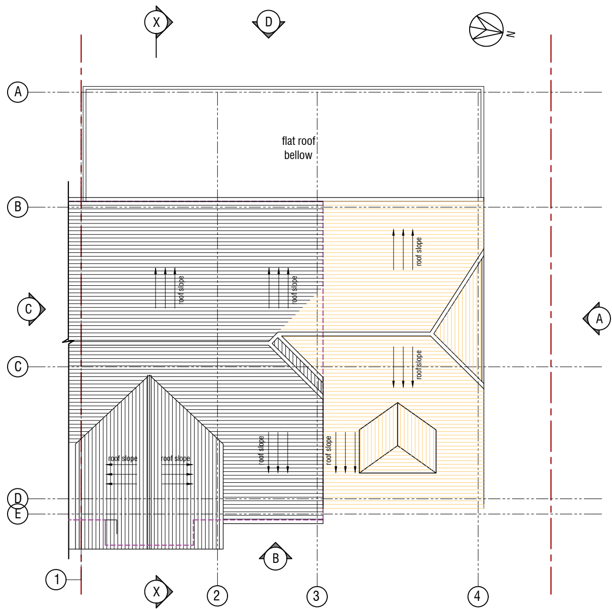
PROPOSED ROOF Scale 1:100
