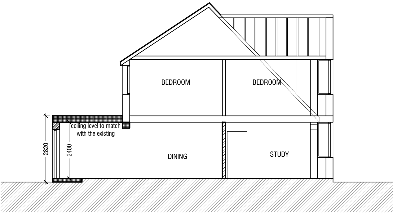
PROPOSED SECTION XX Scale 1:100
