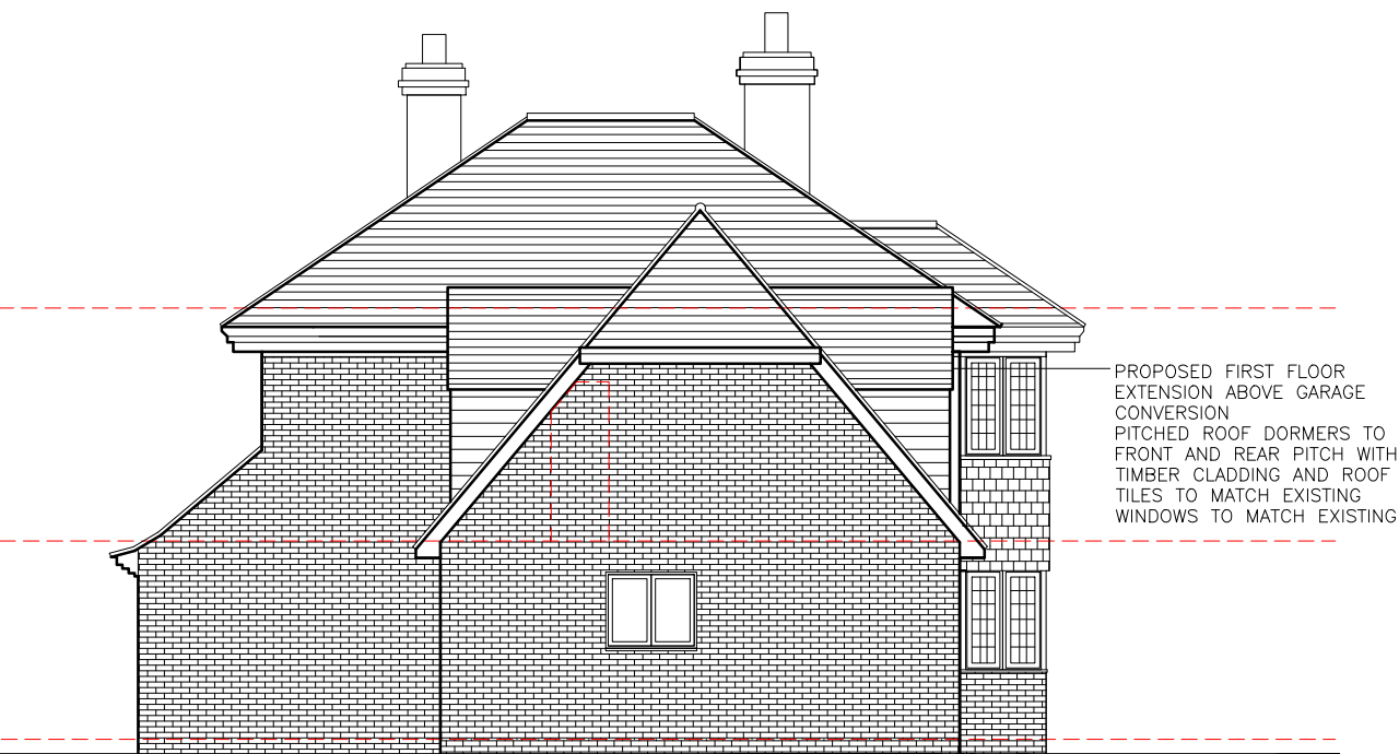
D) Proposed Side Elevation
