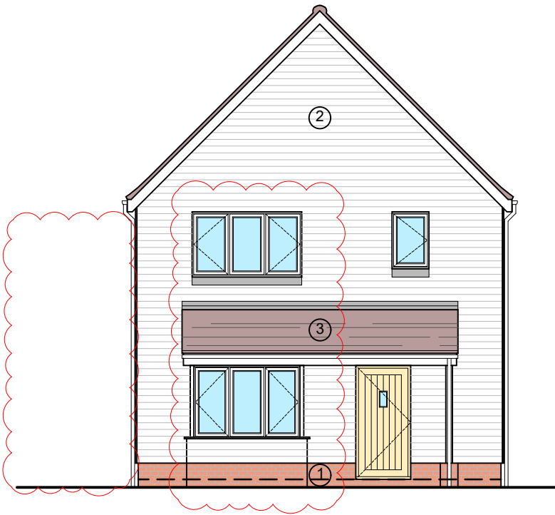
FRONT ELEVATION
