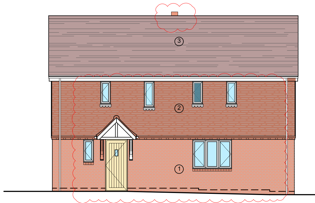
FRONT ELEVATION
