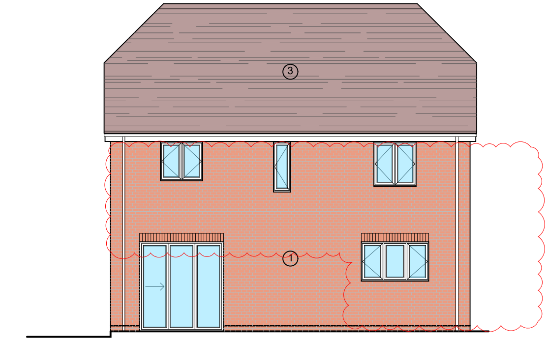
FRONT ELEVATION
