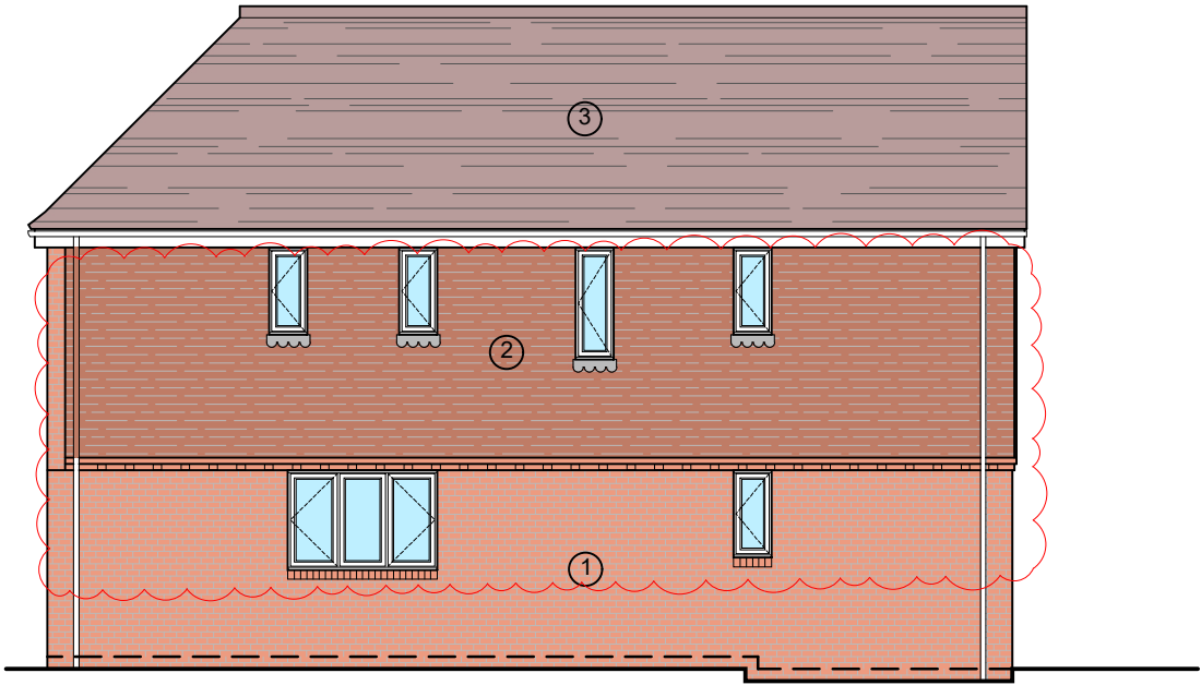
SIDE ELEVATION
