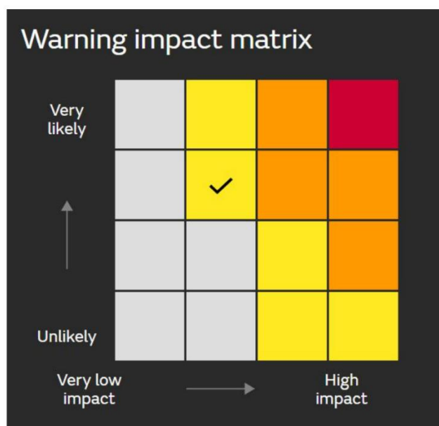
Figure 23: Met Office Weather Warning Impact Matrix (Source: Met Office)
