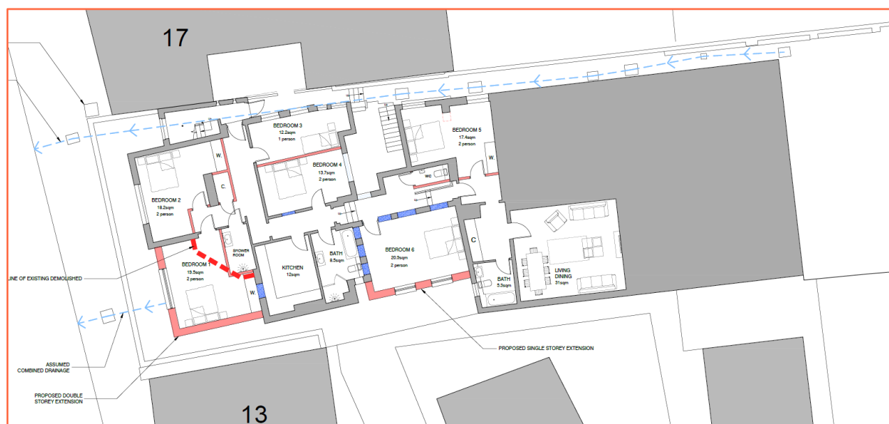
Figure 5: Proposed first floor plan (Source: Applicant)
