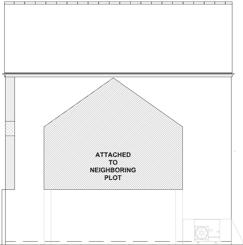
Rear Elevation
