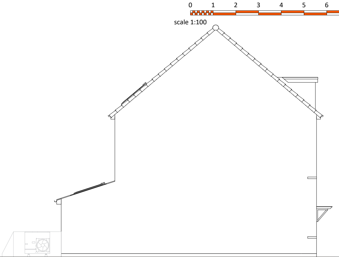
Side Elevation
