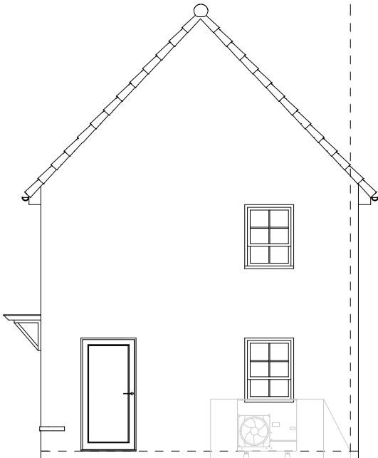
Rear Elevation
