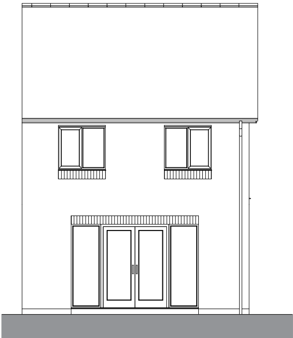
Rear Elevation
