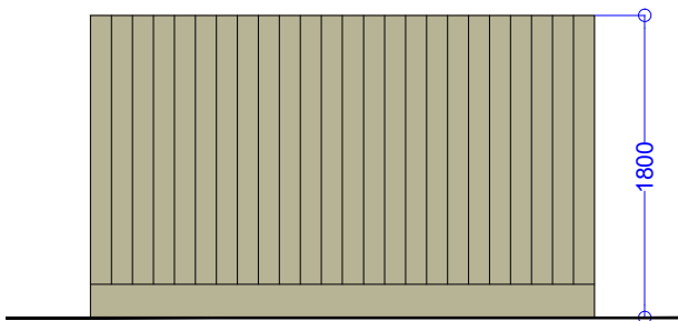
1.8M CLOSE BOARDED FENCE SECTION
