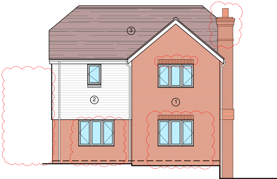
REAR ELEVATION
