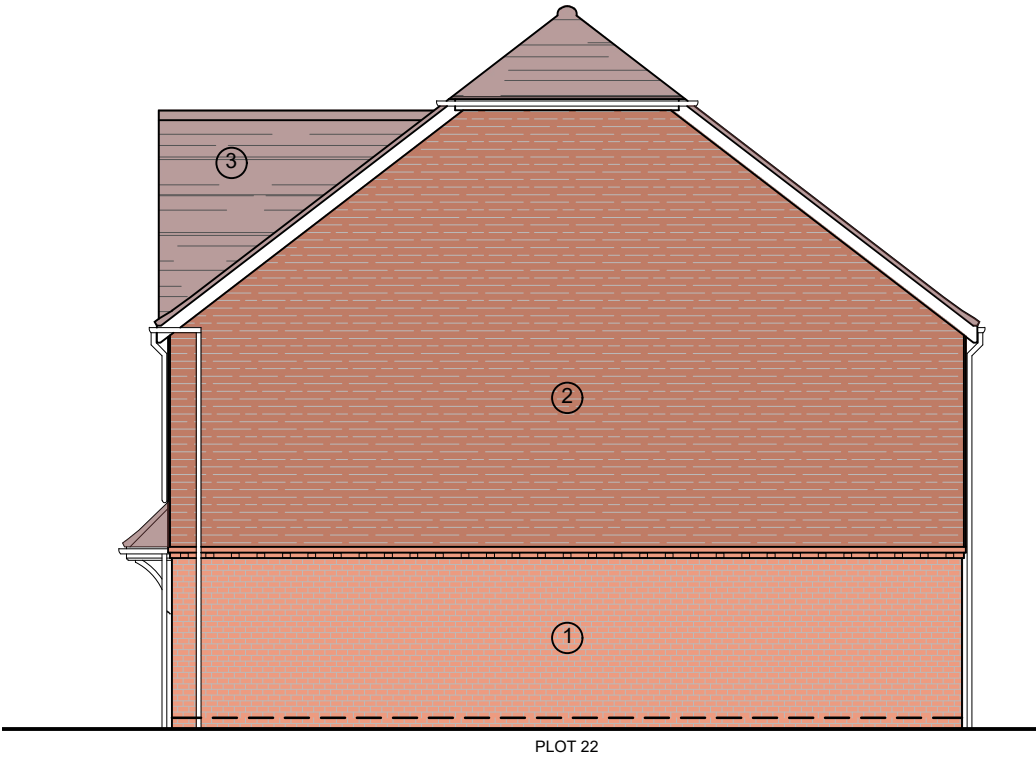
SIDE ELEVATION
