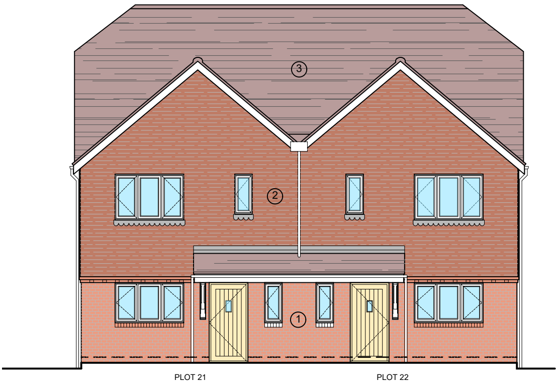
FRONT ELEVATION
