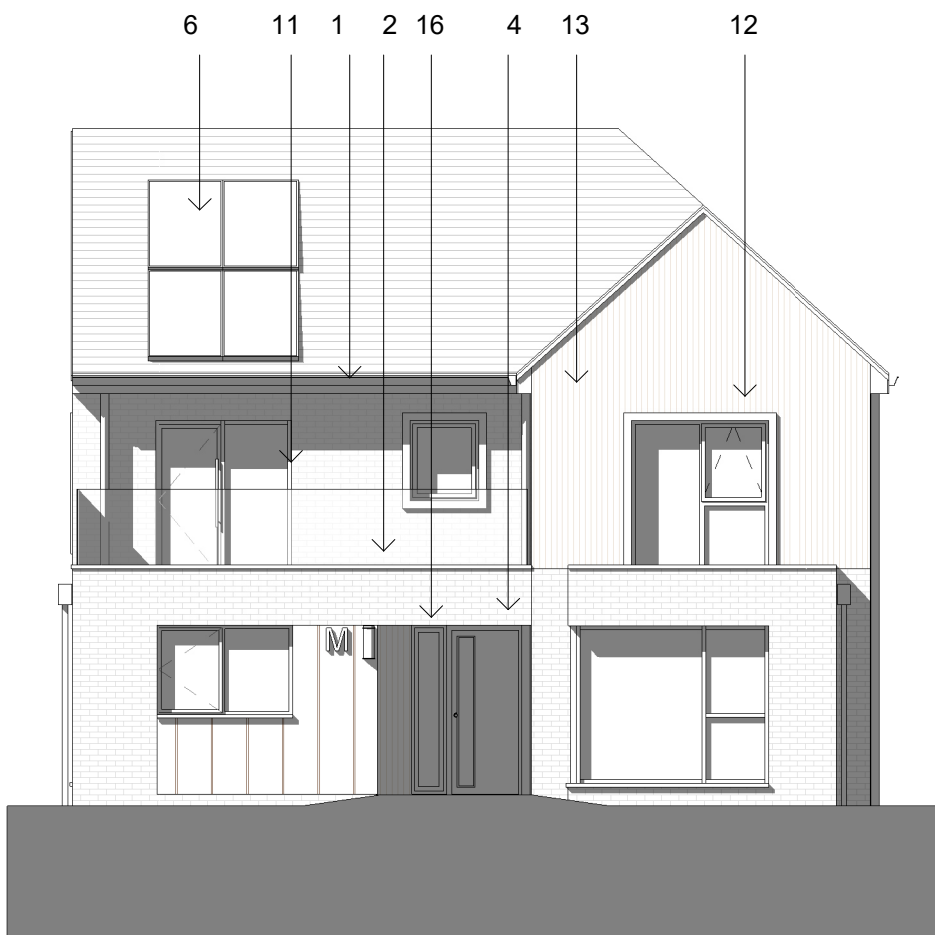
Front Elevation 01 1 : 100
