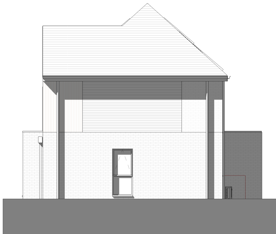
Side Elevation 1 1 : 100
