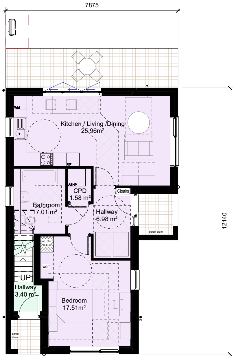
00 Ground FFL 1 : 100
