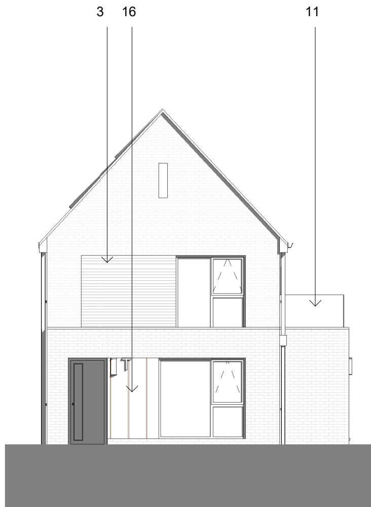
Side Elevation 1 1 : 100
