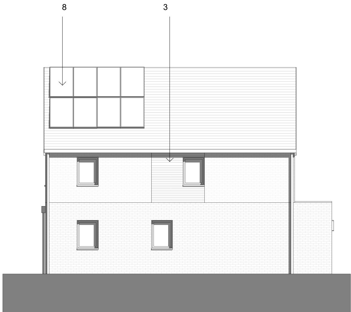
Side Elevation 2 1 : 100
