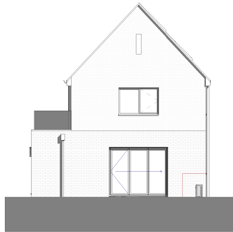
Rear Elevation 1 : 100
