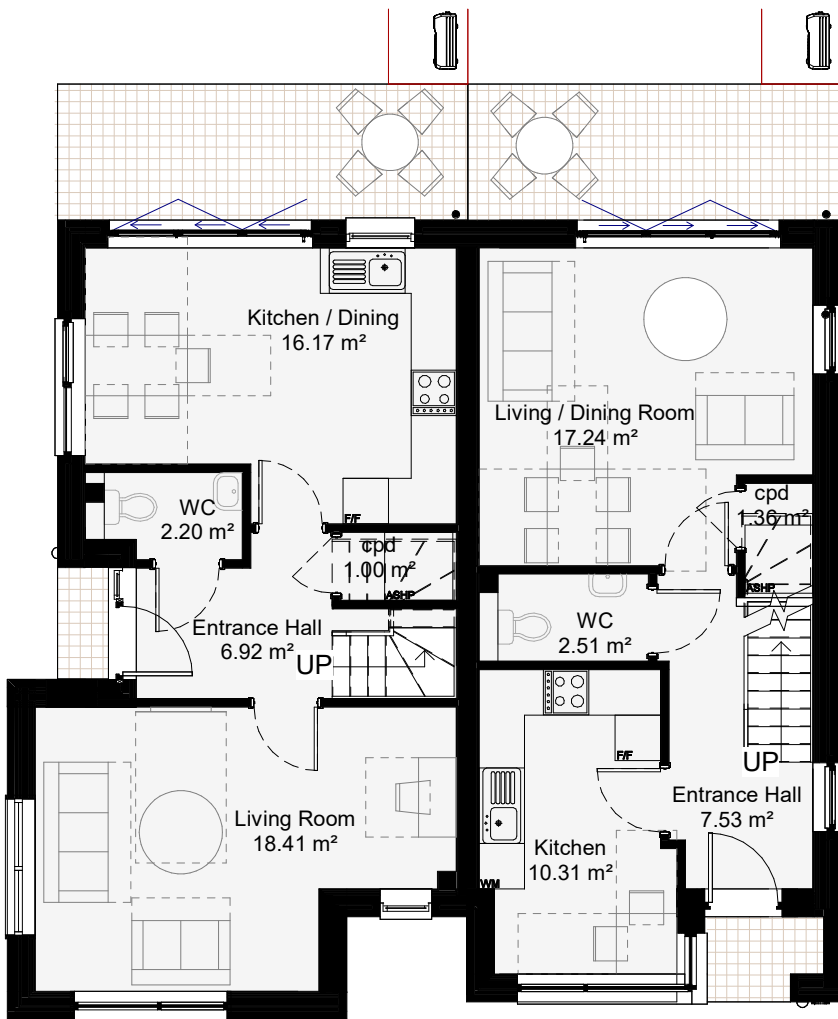
00 Ground FFL 1 : 100
