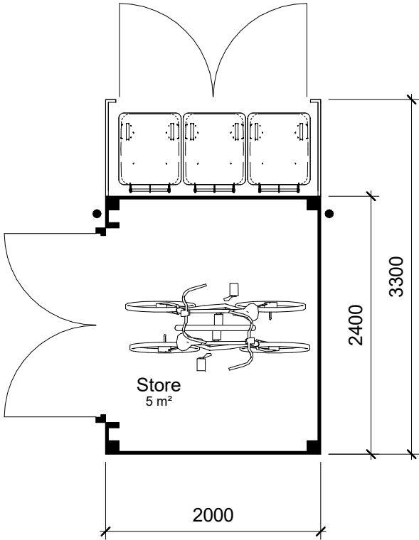
Ground Plan 1 : 50
