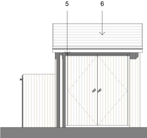
Side Elevation 1 1 : 50
