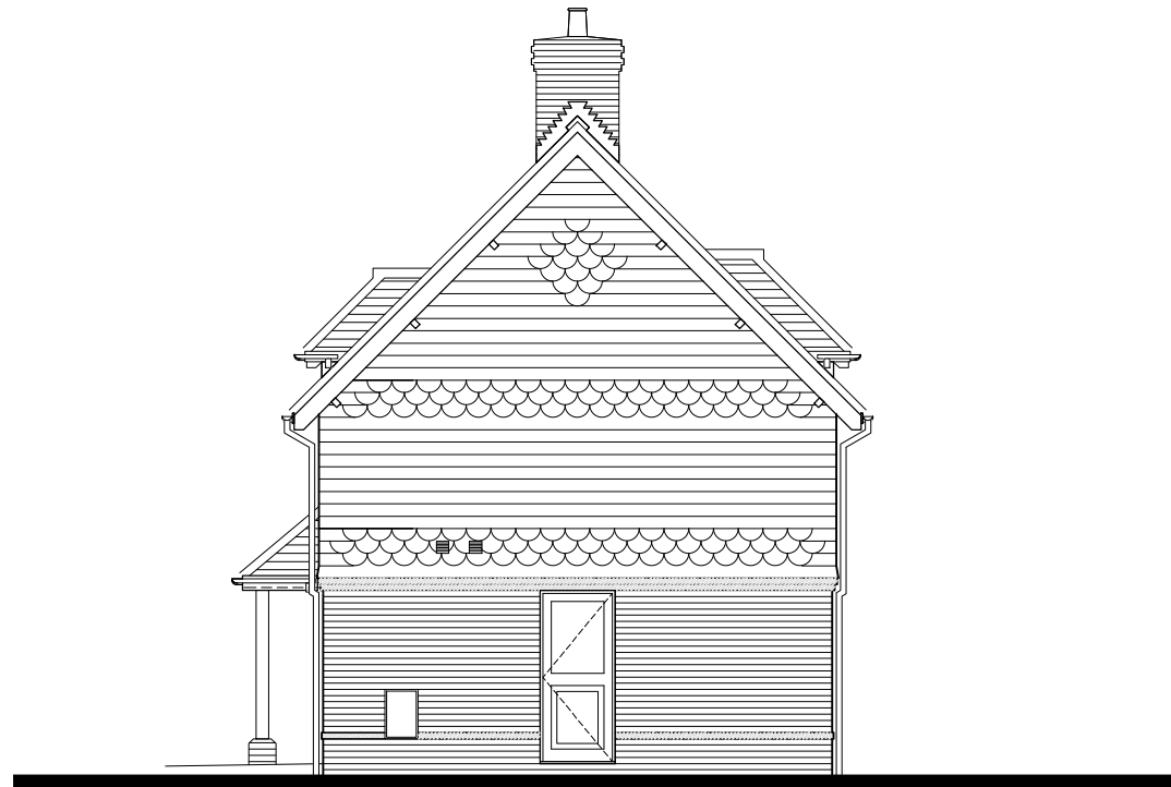
West Elevation
