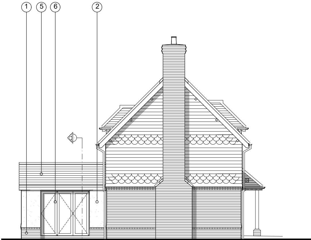
West Elevation
