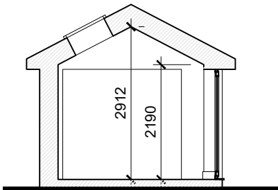
Extension Section
