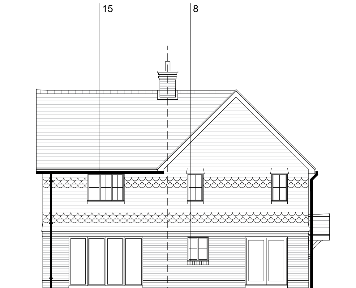
REAR ELEVATION
