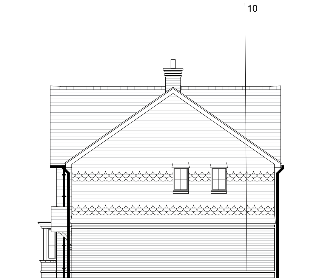
SIDE ELEVATION
