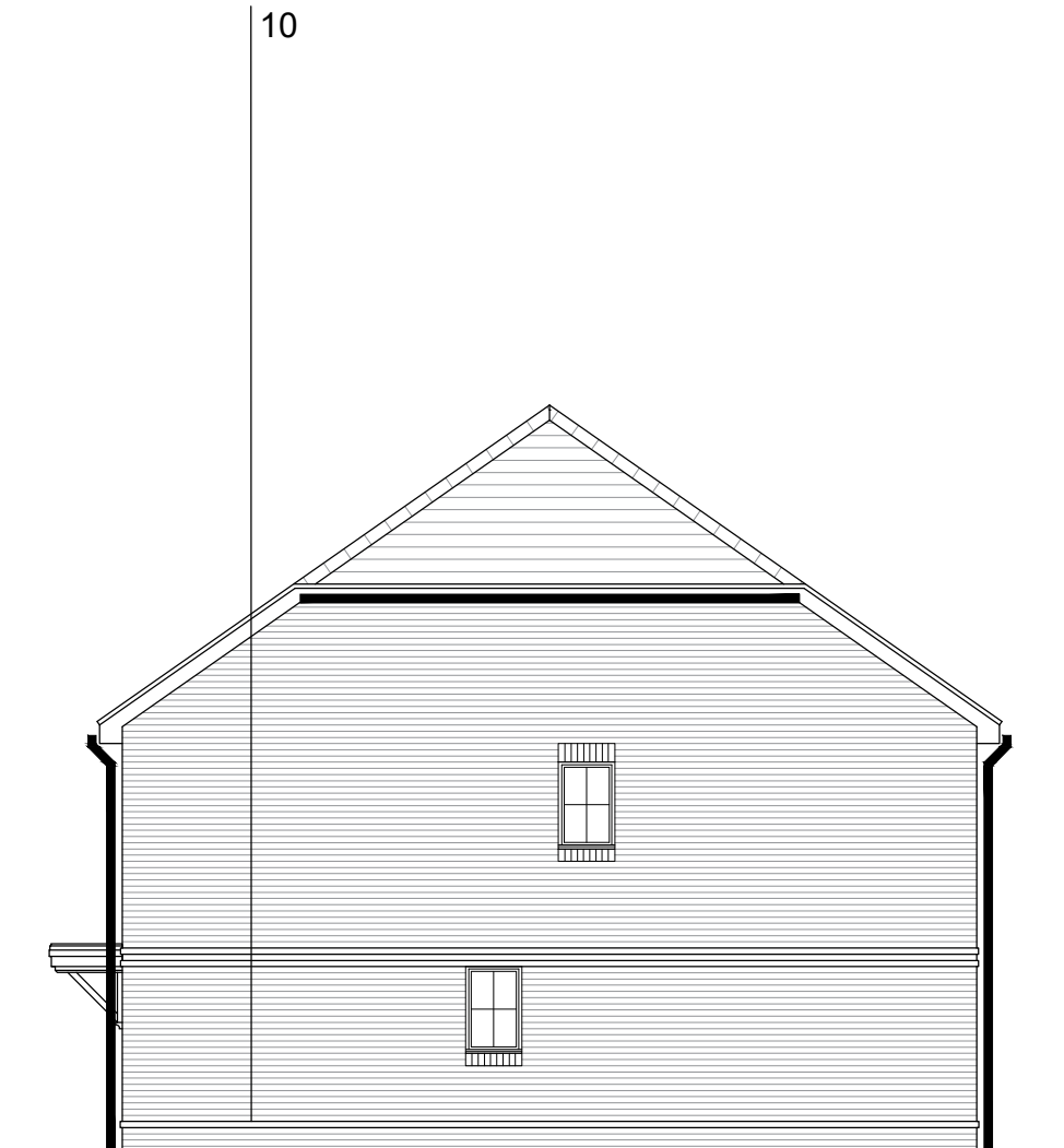
SIDE ELEVATION
