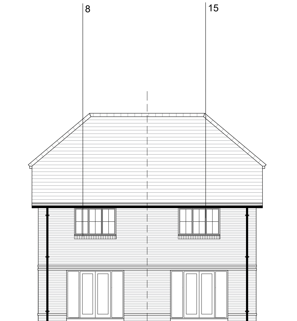
REAR ELEVATION
