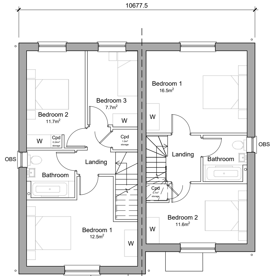
FIRST FLOOR
