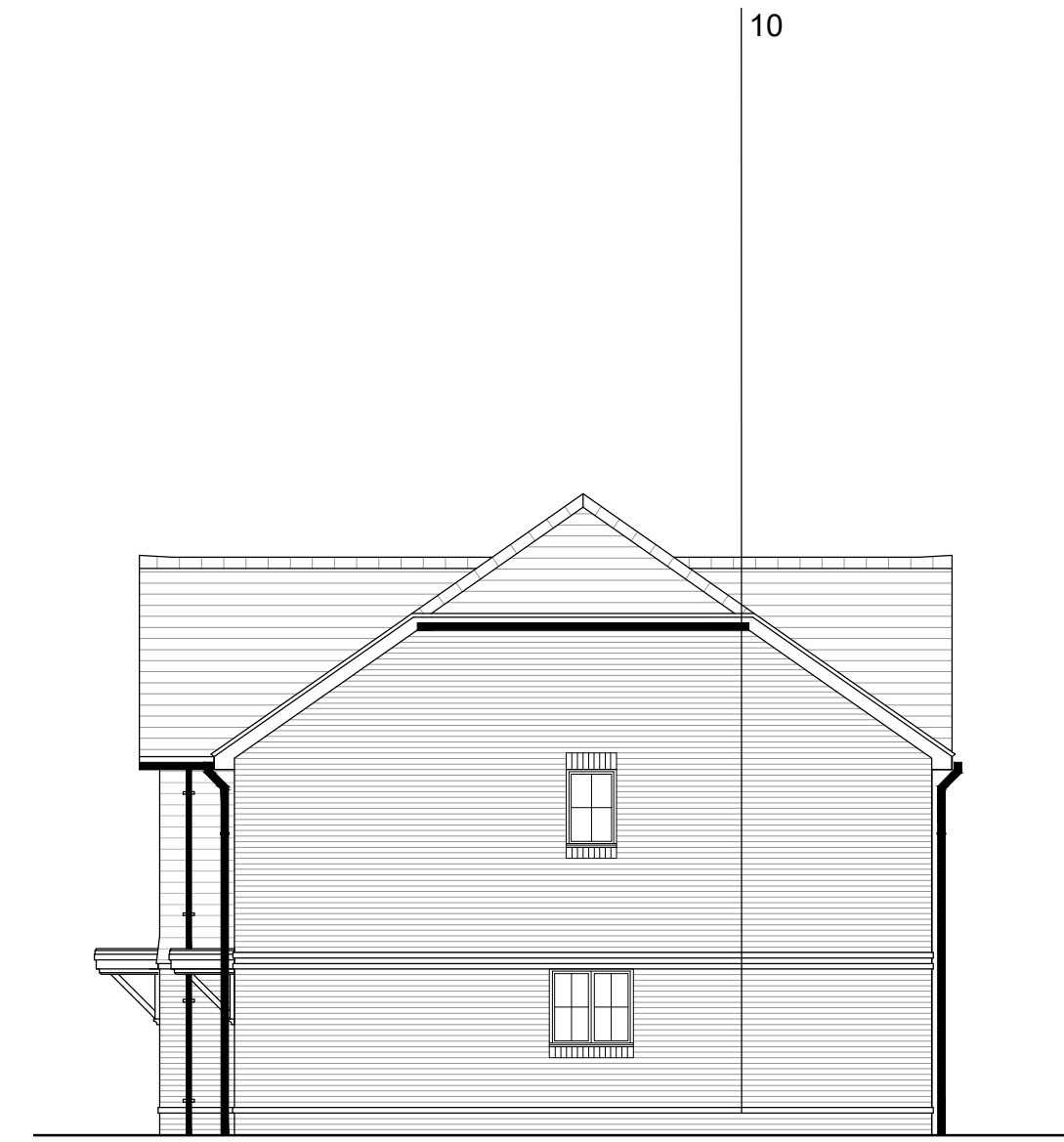
SIDE ELEVATION
