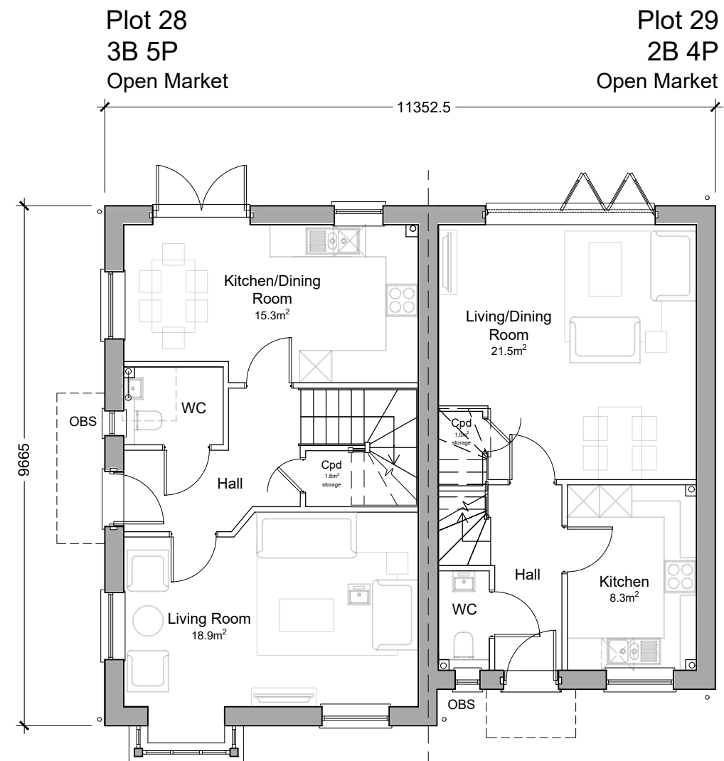
GROUND FLOOR
