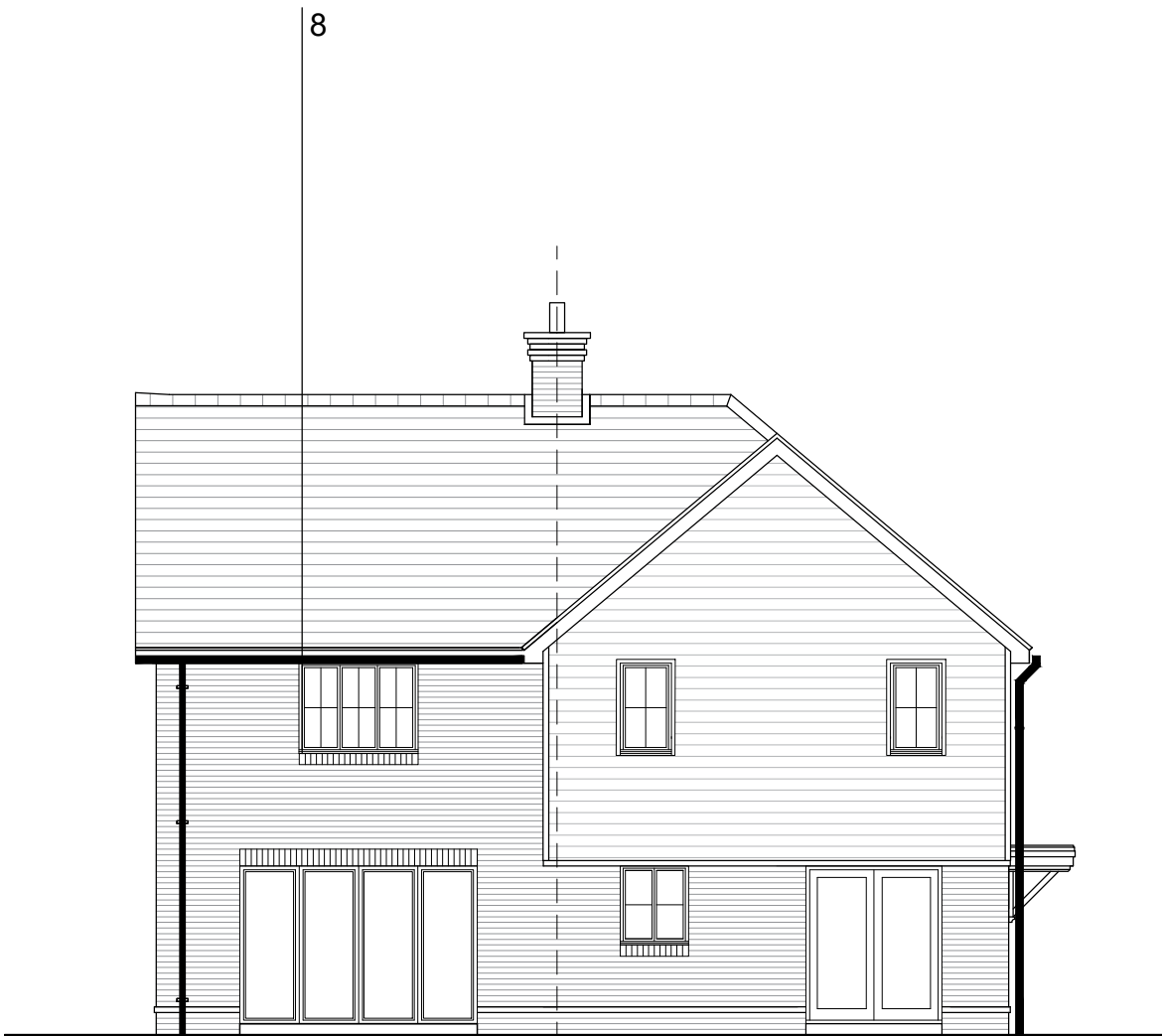
REAR ELEVATION
