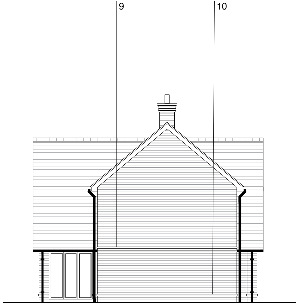
SIDE ELEVATION
