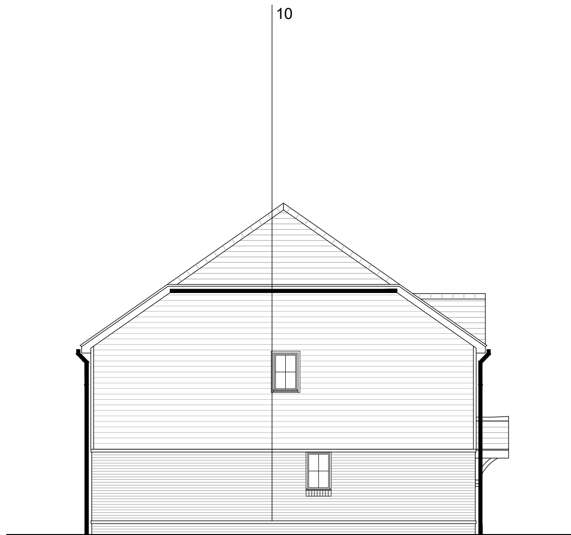
SIDE ELEVATION
