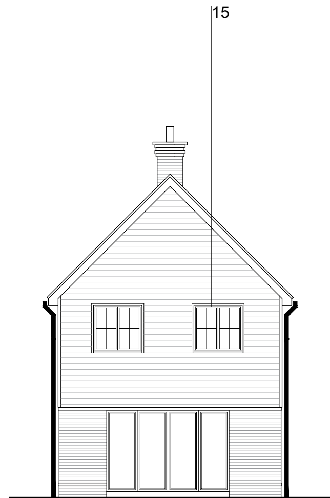
REAR ELEVATION
