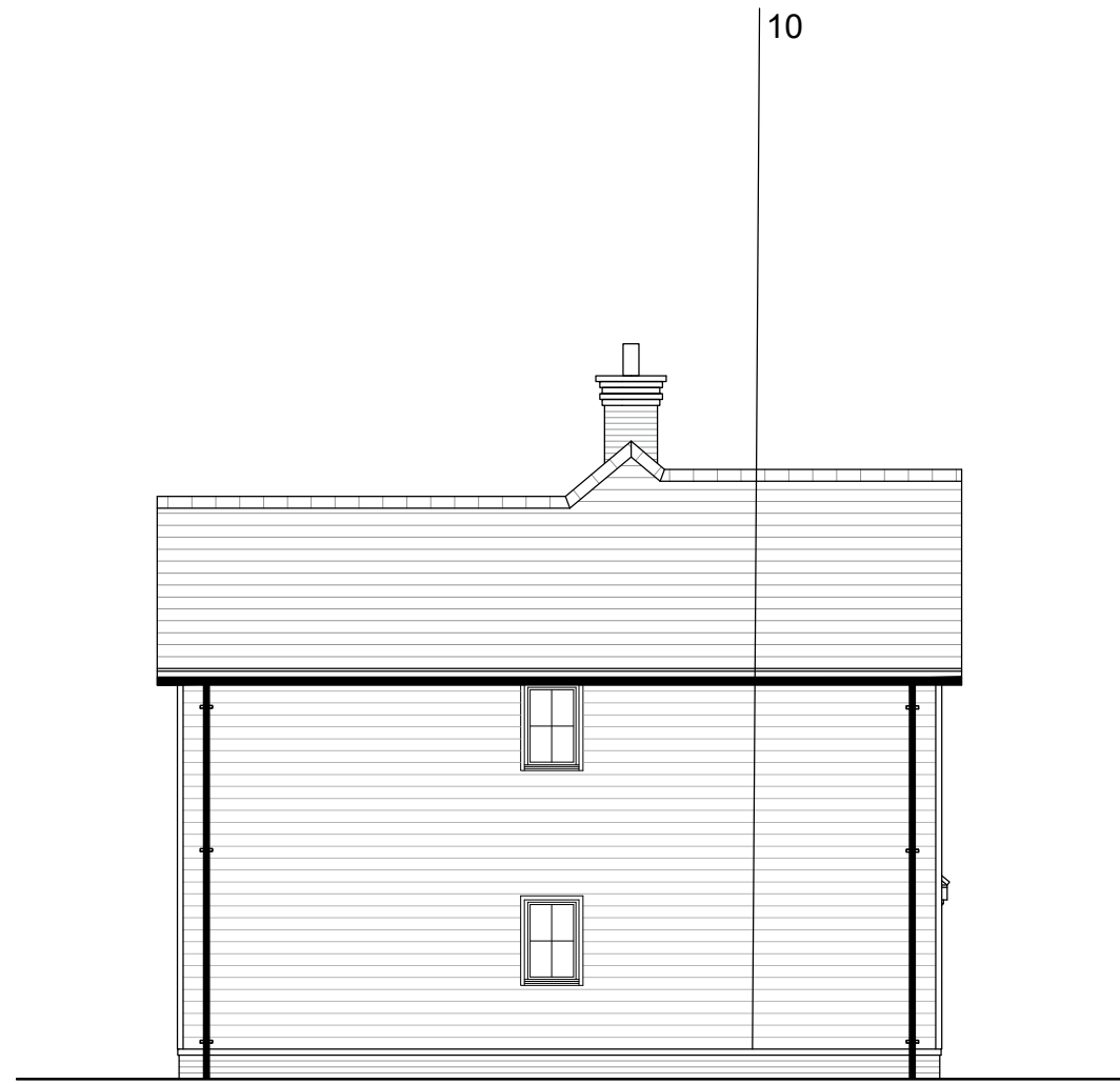
SIDE ELEVATION
