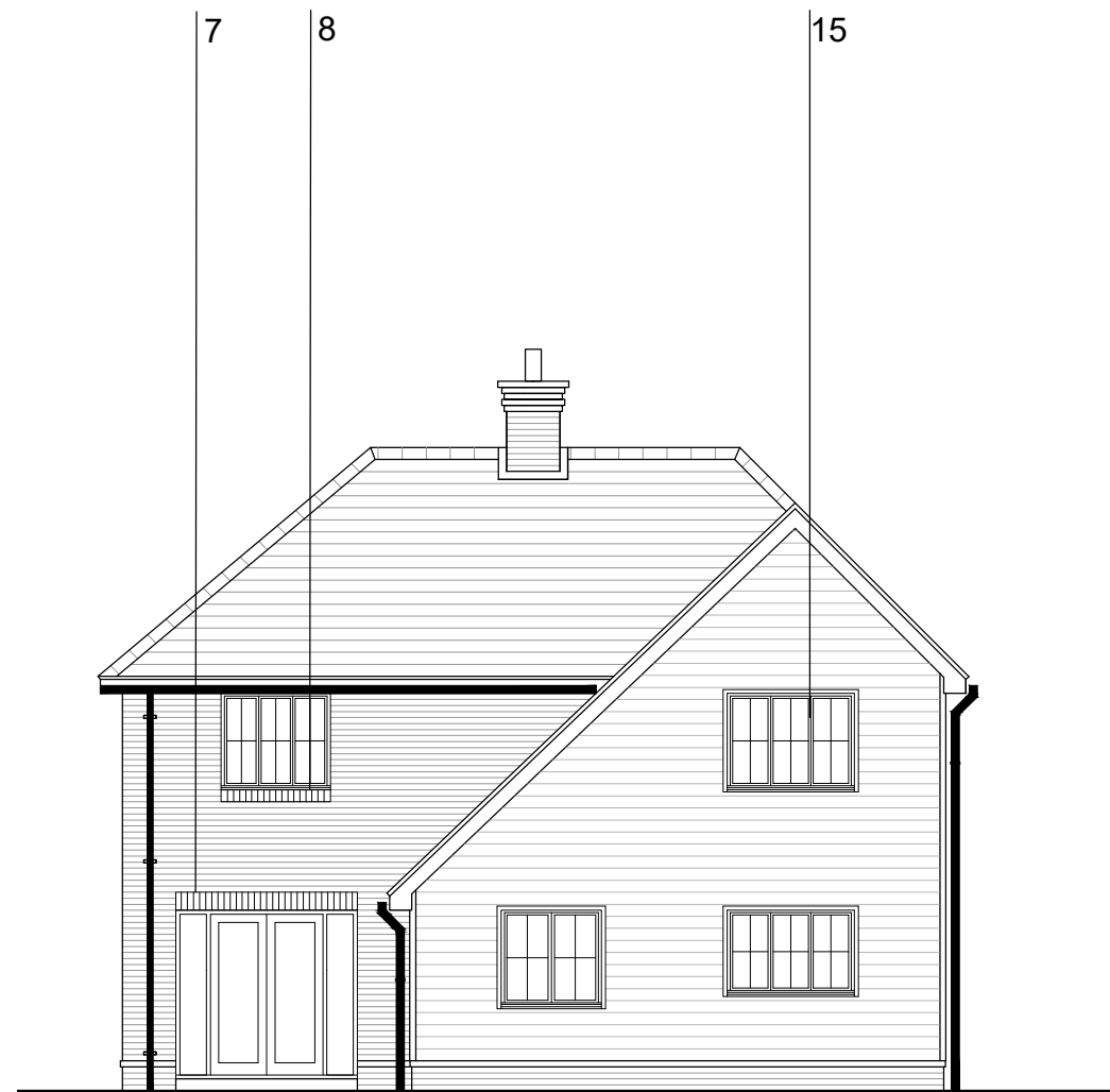
REAR ELEVATION
