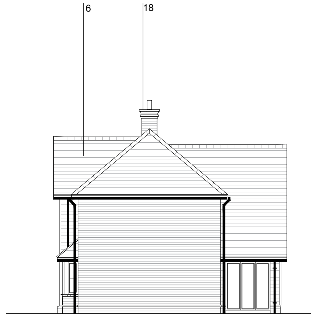
SIDE ELEVATION
