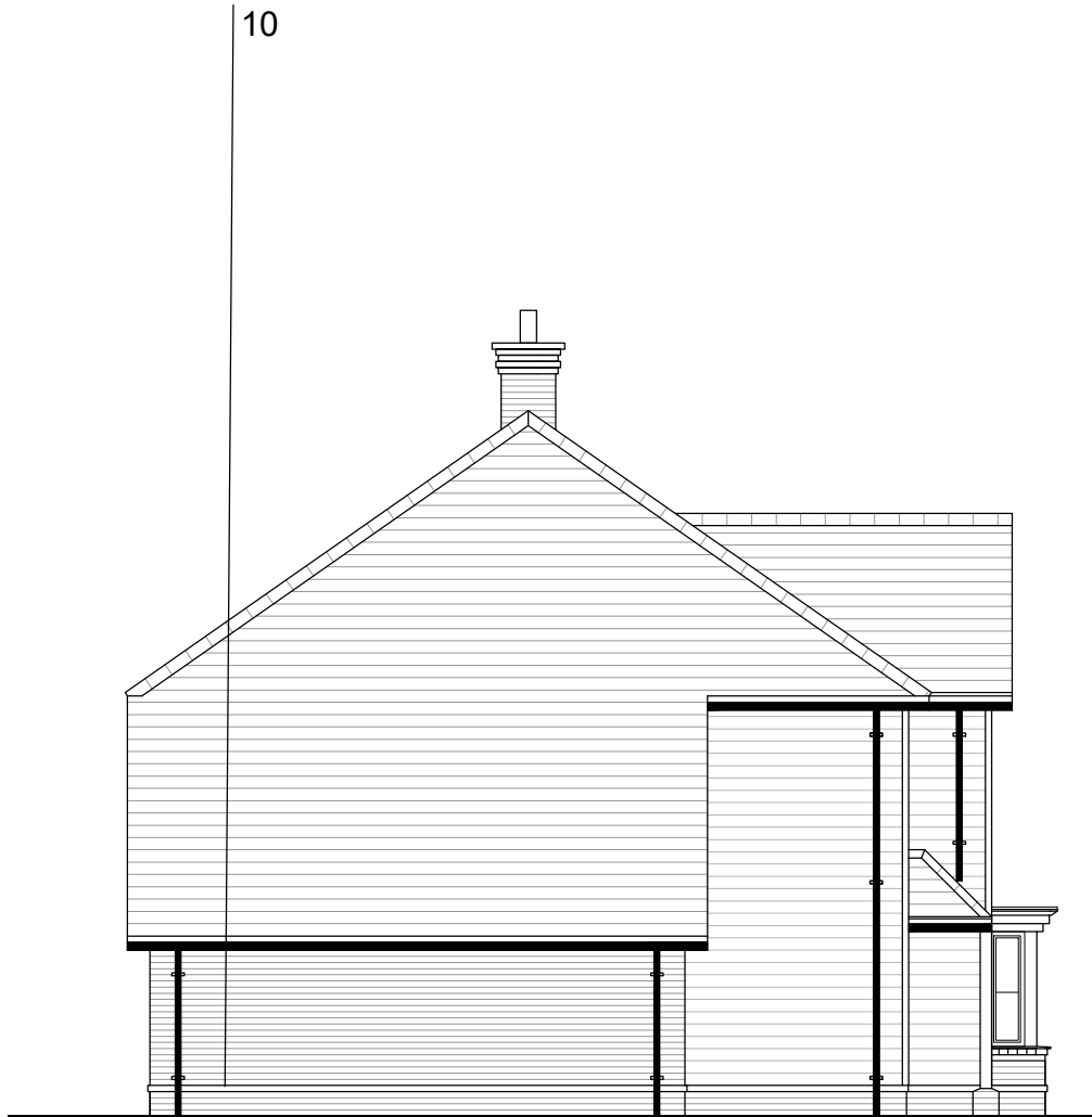
SIDE ELEVATION
