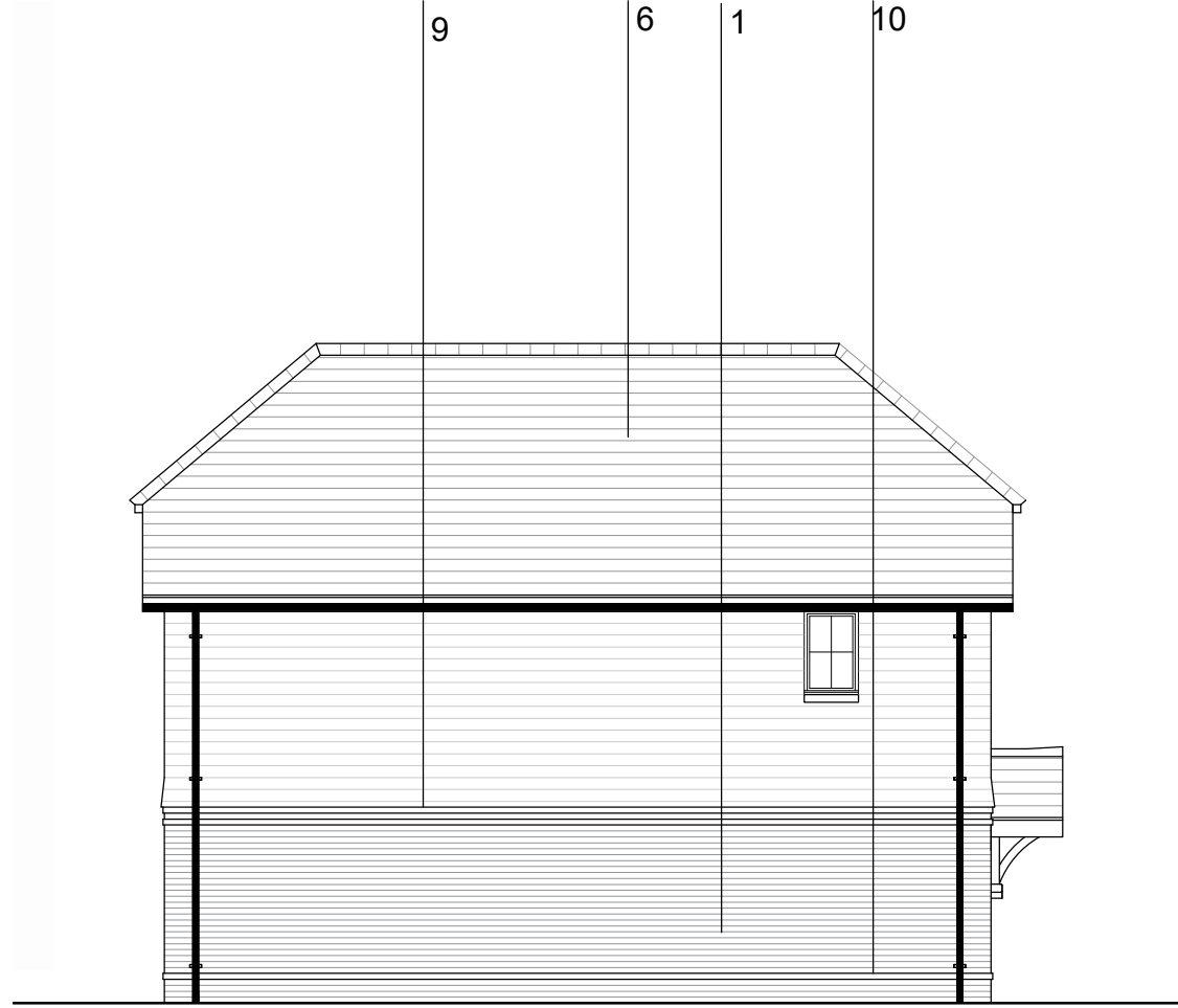
SIDE ELEVATION
