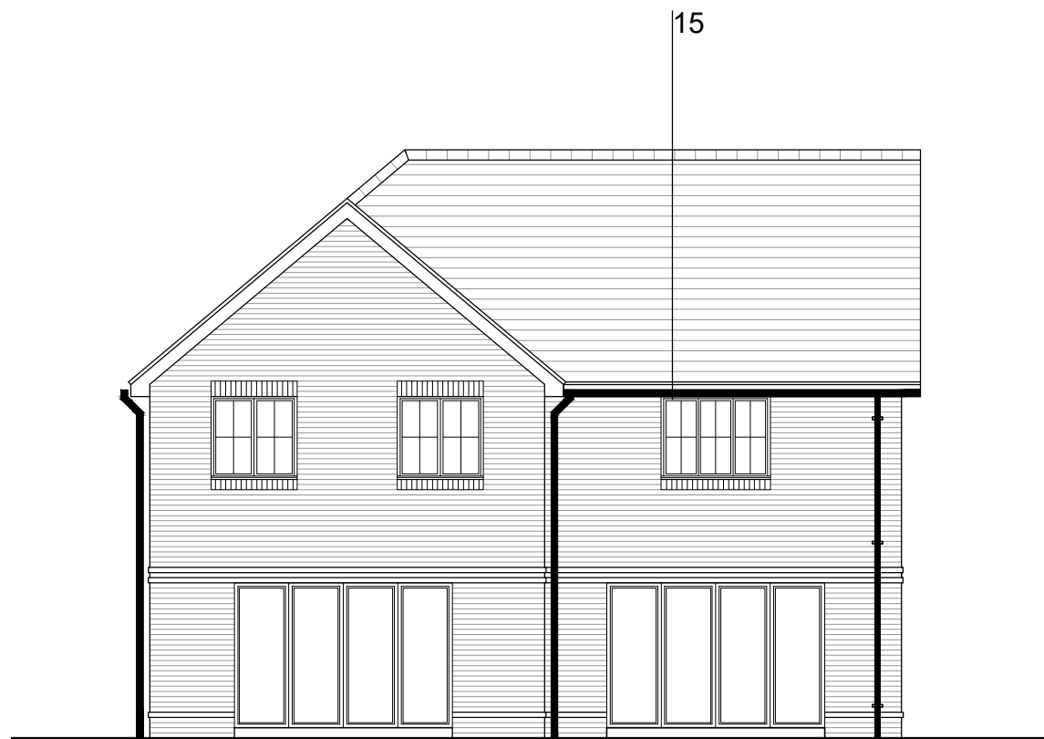
REAR ELEVATION
