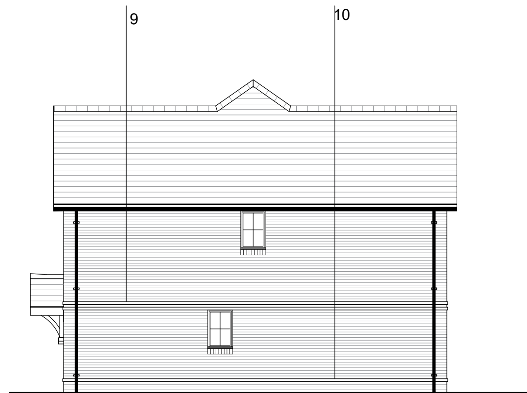
SIDE ELEVATION
