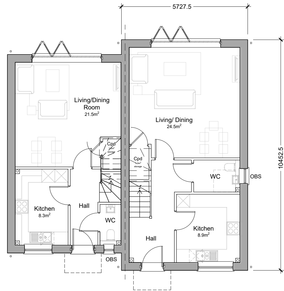
GROUND FLOOR
