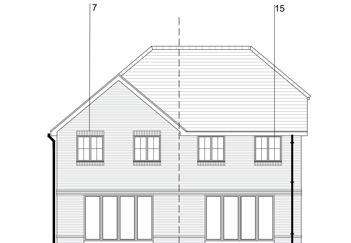
REAR ELEVATION
