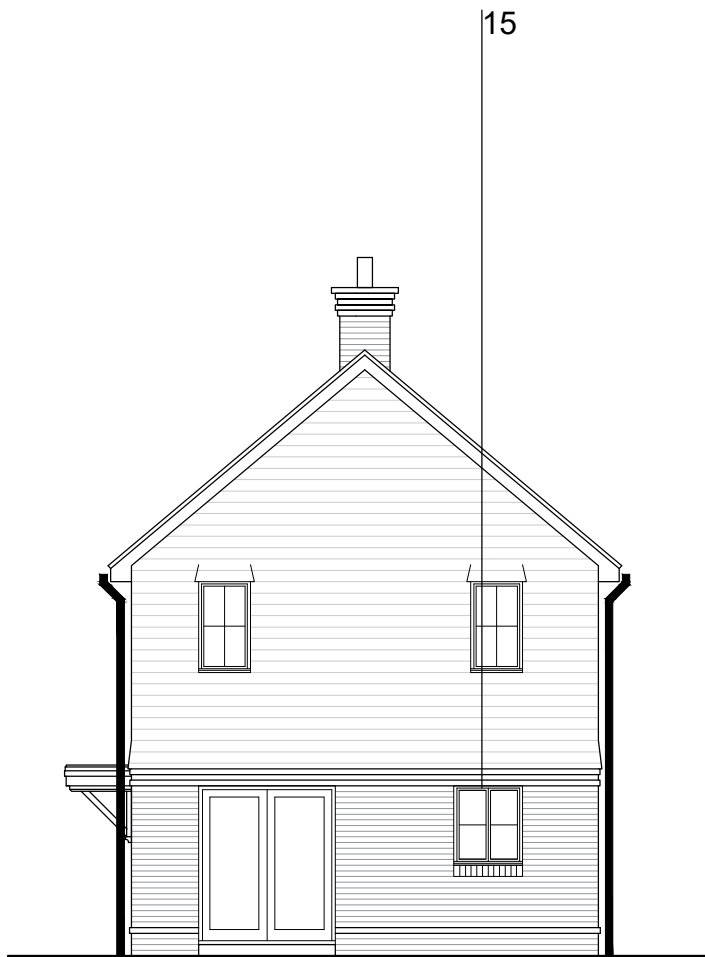
SIDE ELEVATION
