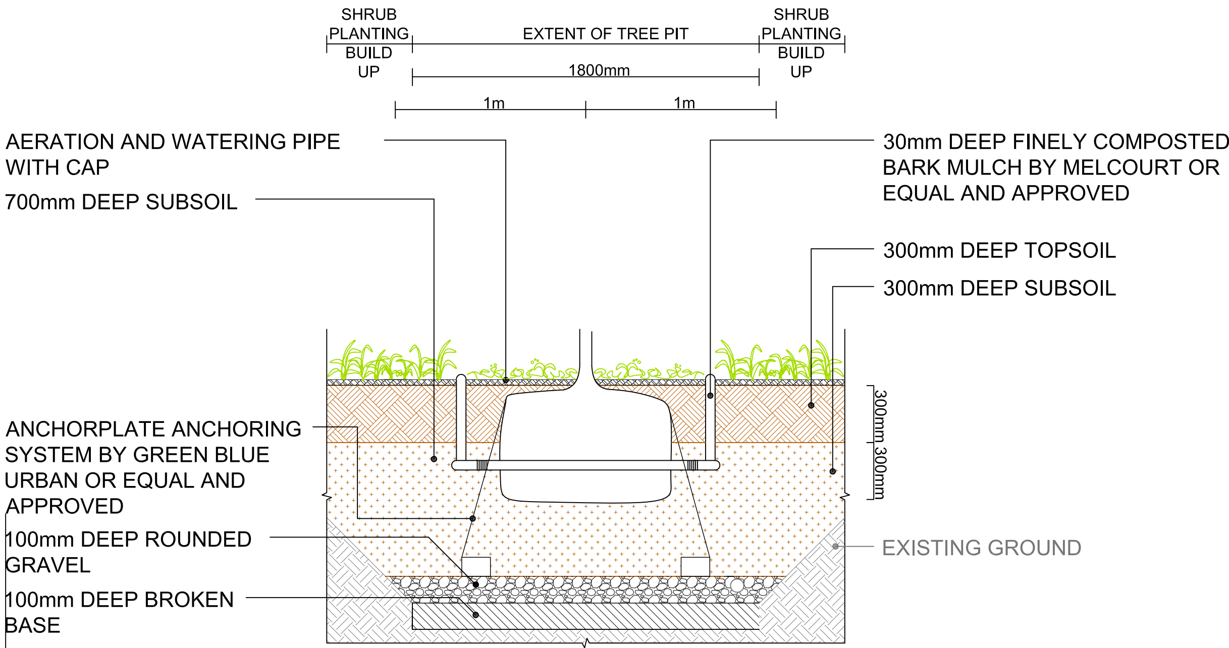
DETAIL 9.01 A TREE PIT IN SOFT LANDSCAPE SCALE 1:20
