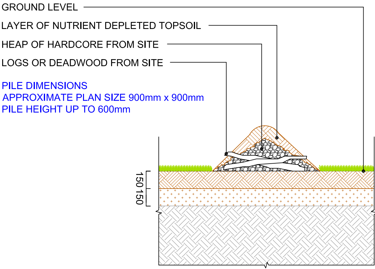
DETAIL 9.01 G INVERTEBRATE SPOIL PILE BUILD UP SCALE 1:20
