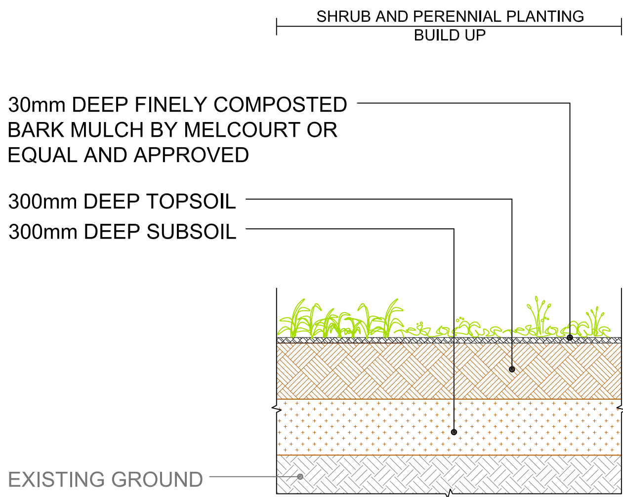
DETAIL 9.01 B ORNMENTAL PLANTING IN PROVATE GARDENS SHRUB AND PERENNIAL PLANTING BUILD UP SCALE 1:20
