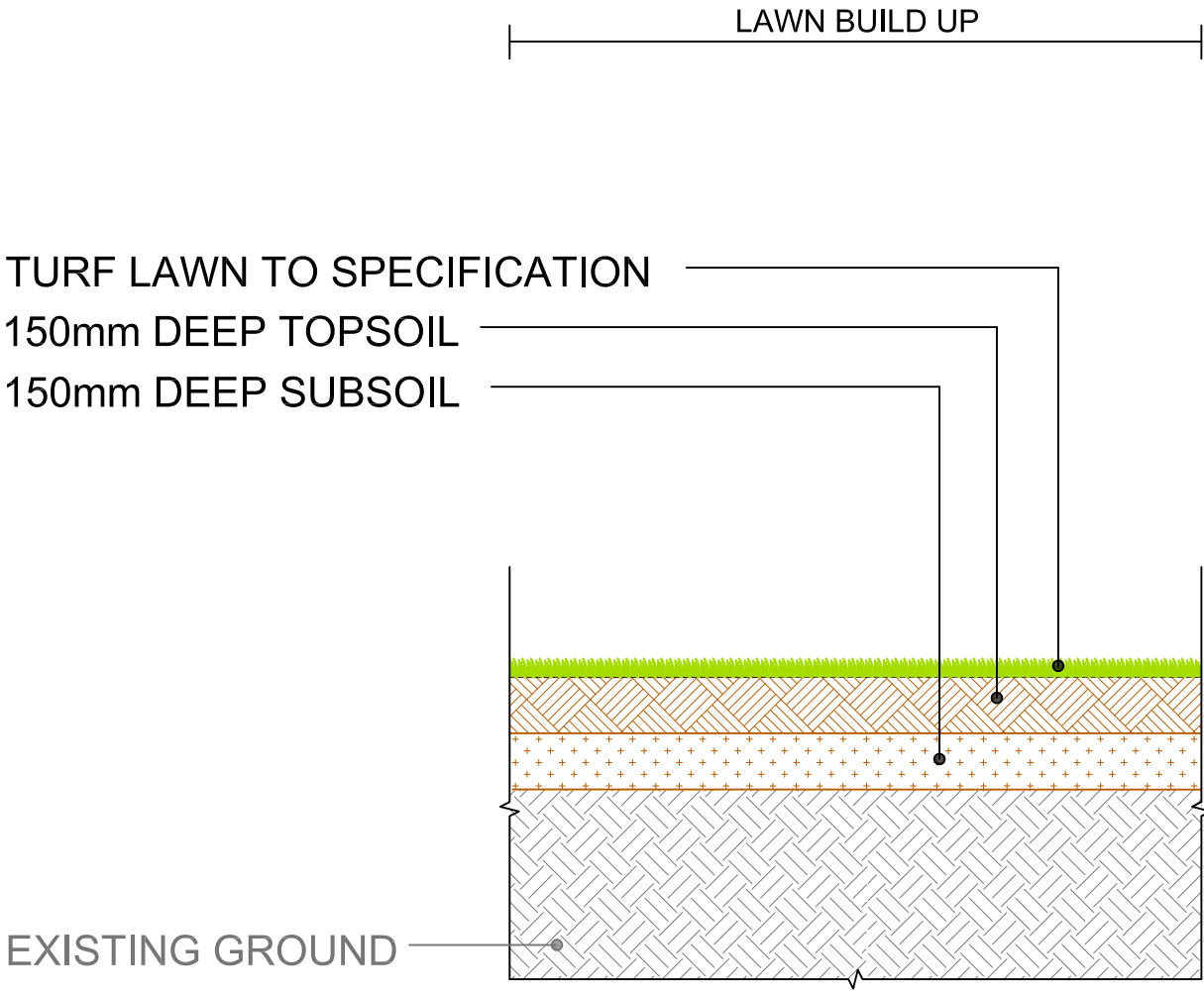
DETAIL 9.01 C LAWN BUILD UP SCALE 1:20
