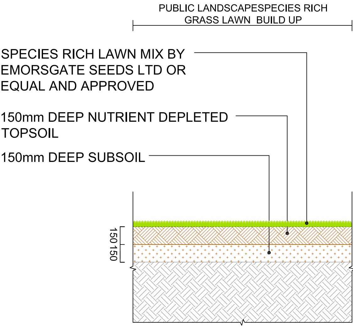
DETAIL 9.01 D PUBLIC REALM SPECIES RICH GRASS LAWN AREA BUILD UP SCALE 1:20
