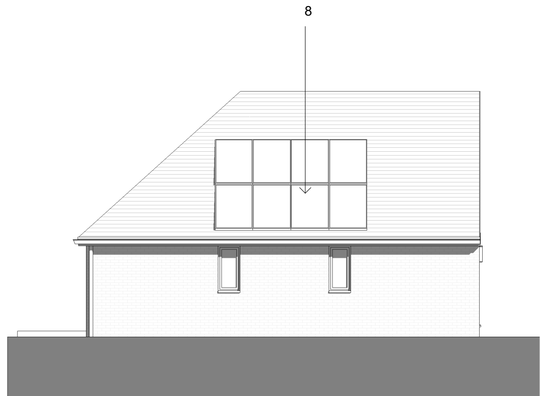
Side Elevation 2 1 : 100
