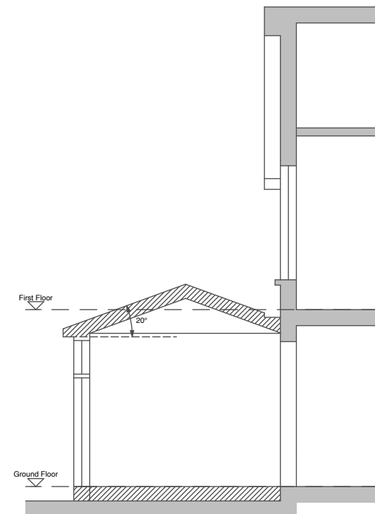
SECTION THROUGH SOUTH/REAR ELEVATION
