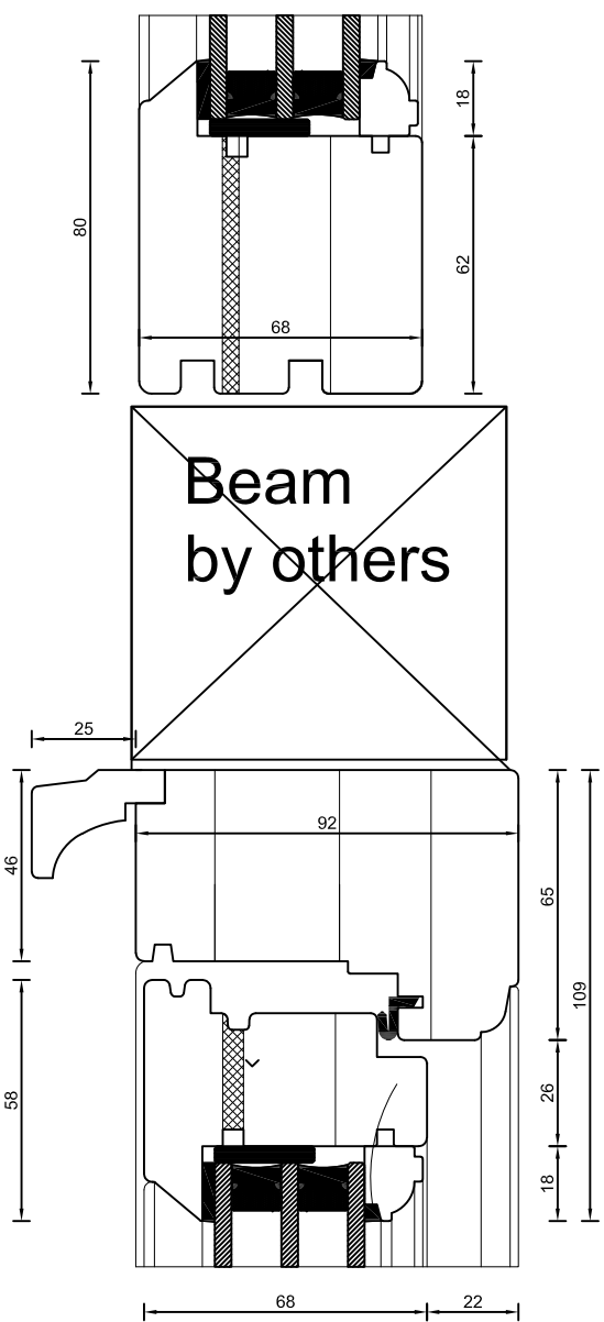
Door Fanlight sections
