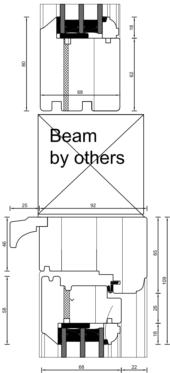
Window Fanlight sections
