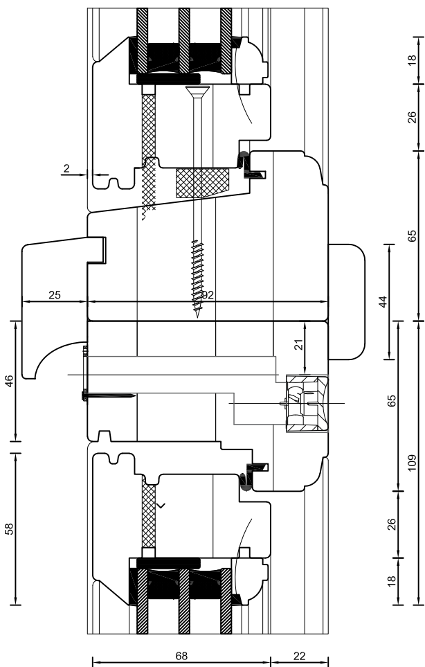
Window head sections
