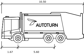
Mid Sussex Refuse Vehicle
