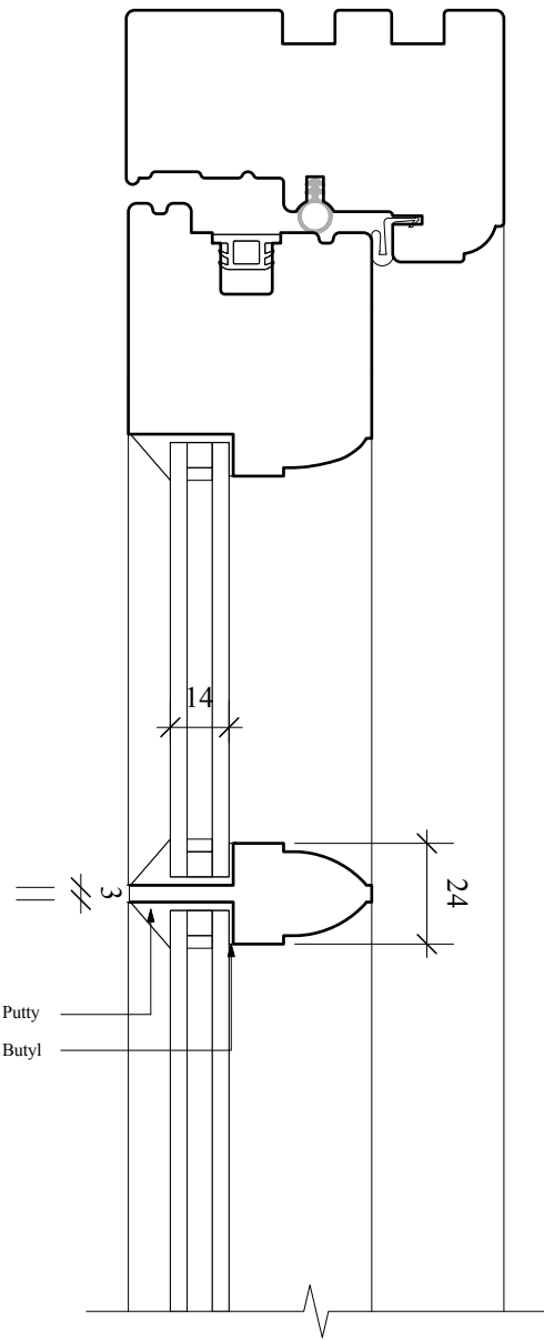
DT-02 Ovolo Glazing Bar - 14 mm double glazed
