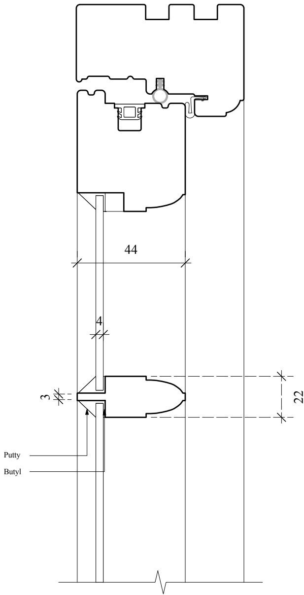
DT-01 Ovolo Glazing Bar - 4mm single glazed
