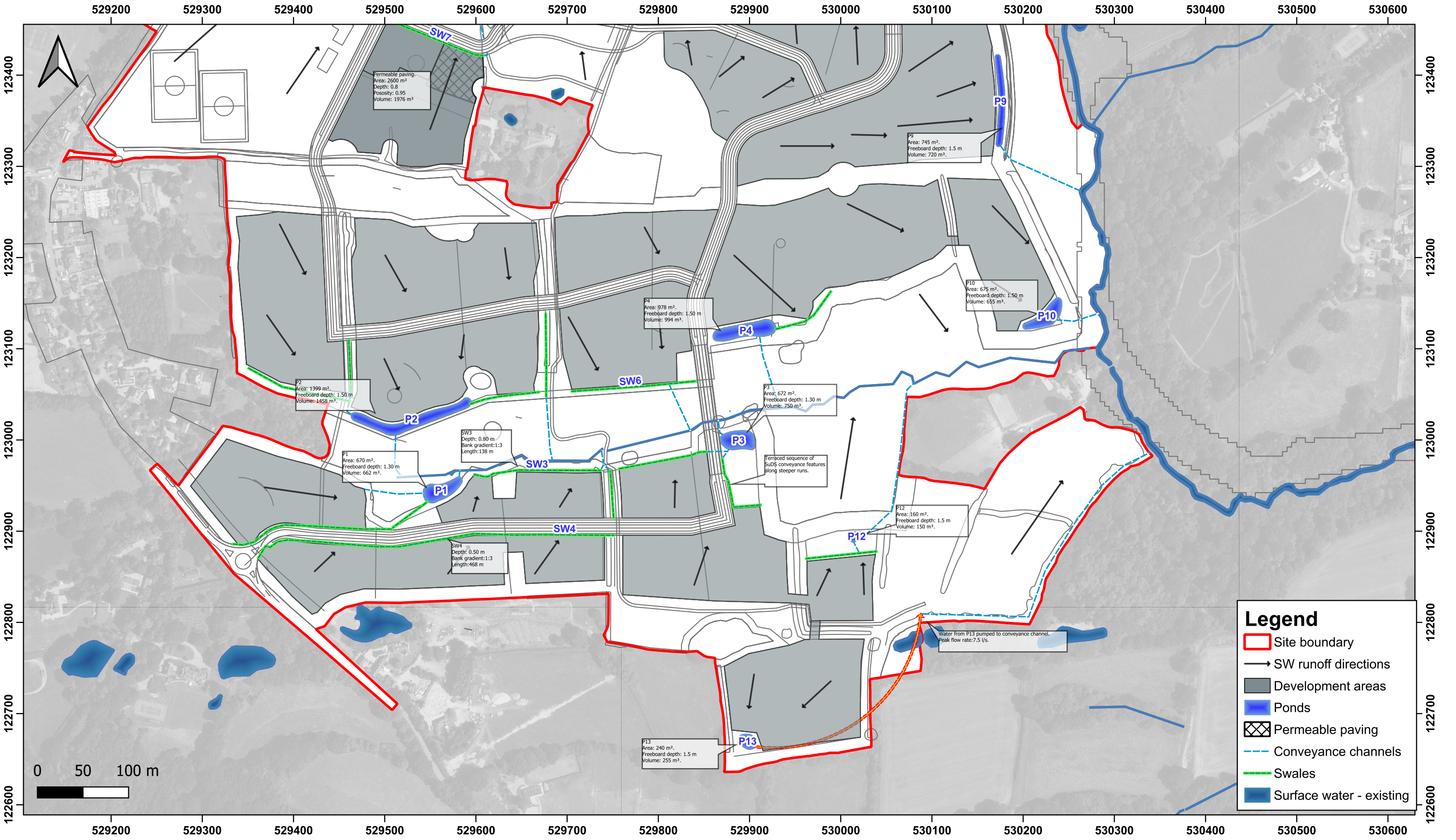
Outline drainage layout and relevant design information.
