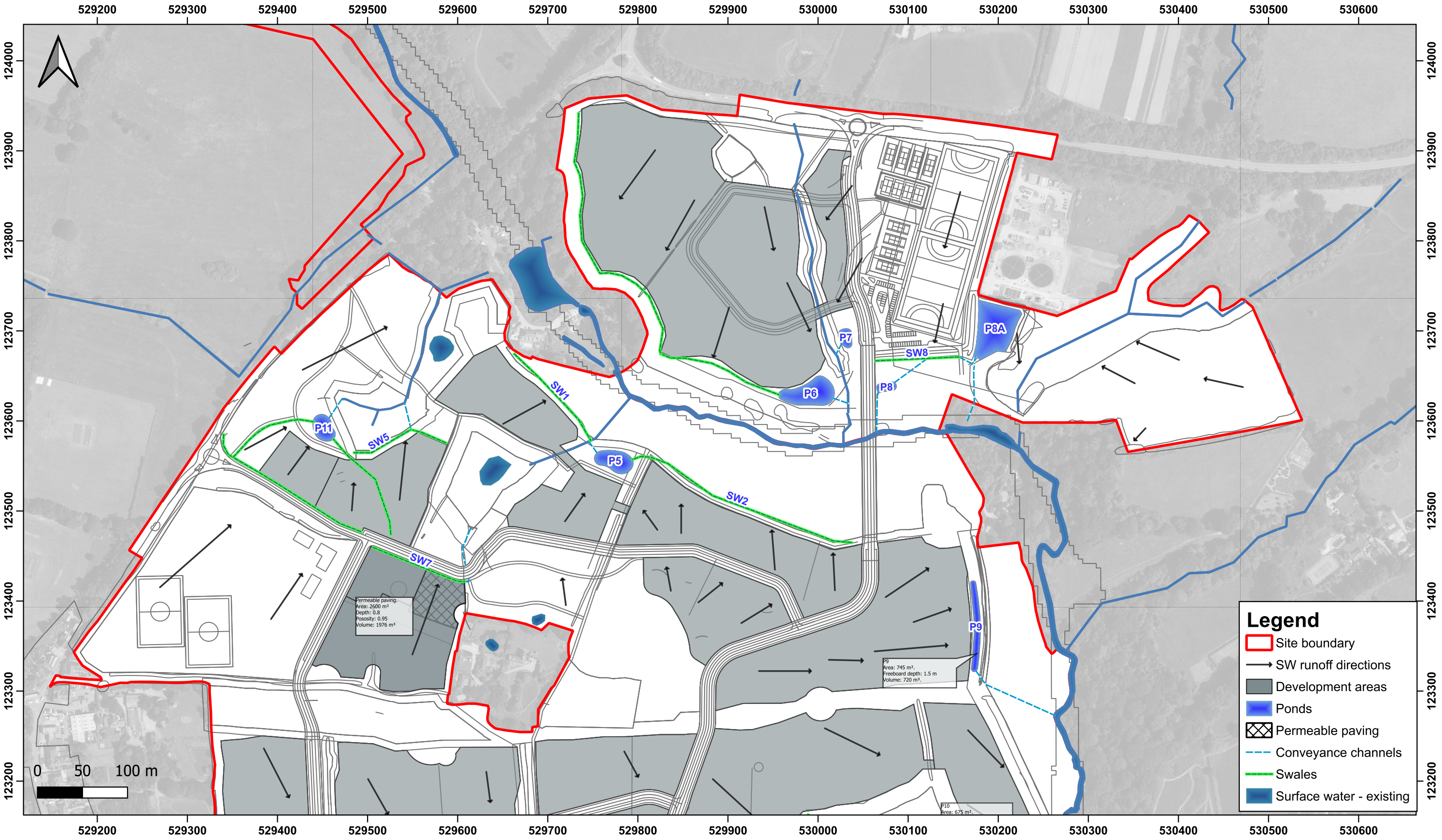
Conceptual drainage layout and relevant design information.
