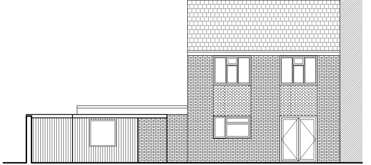
3 EXISTING REAR ELEVATION 1:100
