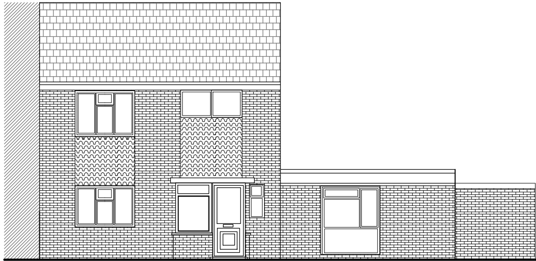
1 EXISTING PRINCIPAL (FRONT) ELEVATION 1:100
