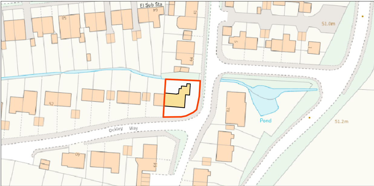
1 EXISTING SITE LOCATION PLAN 1:1250
