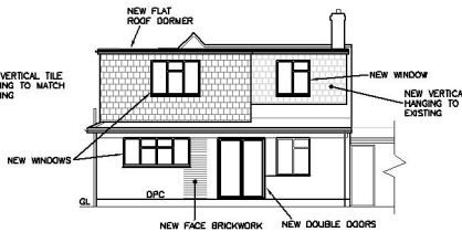
02.08 REAR (SWW) ELEVATION AS PROPOSED
