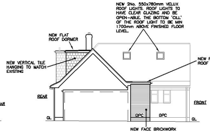
02.10 SIDE (SSE) ELEVATION AS PROPOSED
