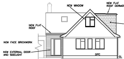
02.07 FRONT (NEE) ELEVATION AS PROPOSED
