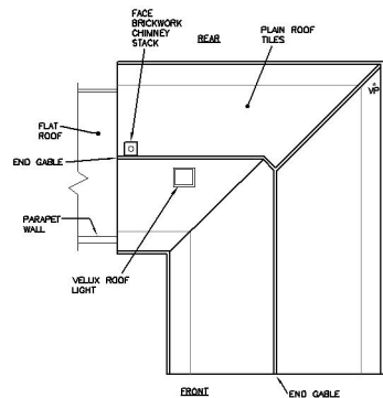
02.01 – ROOF PLAN AS EXISTING
