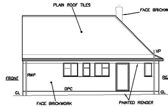
02.05 SIDE (NNW) ELEVATION AS EXISTING
