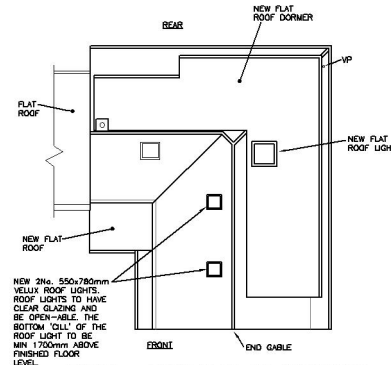
02.02 – ROOF PLAN AS PROPOSED
