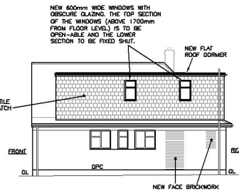
02.09 SIDE (NNW) ELEVATION AS PROPOSED
