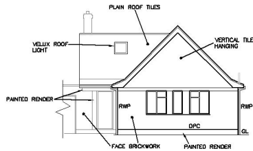
02.03 FRONT (NEE) ELEVATION AS EXISTING
