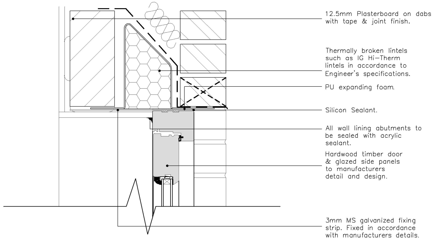
DOOR SECTION HEAD DETAIL
