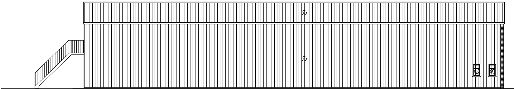
West elevation
