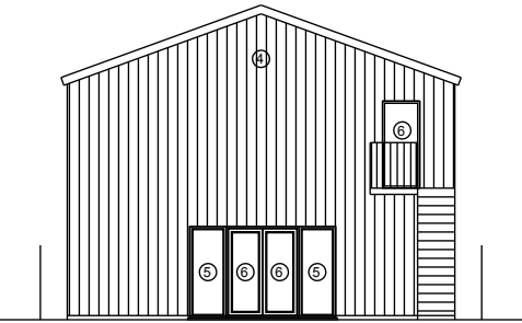
North elevation
