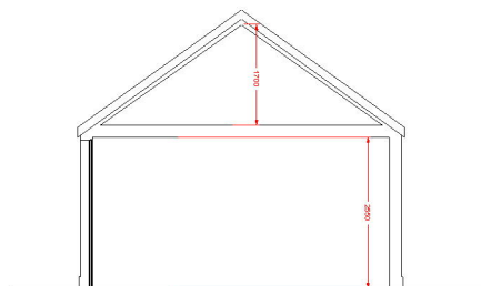
Section 1:50
