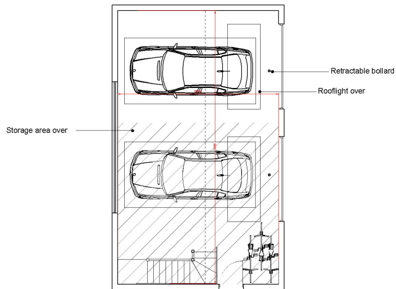
Ground Floor Plan 1:50
