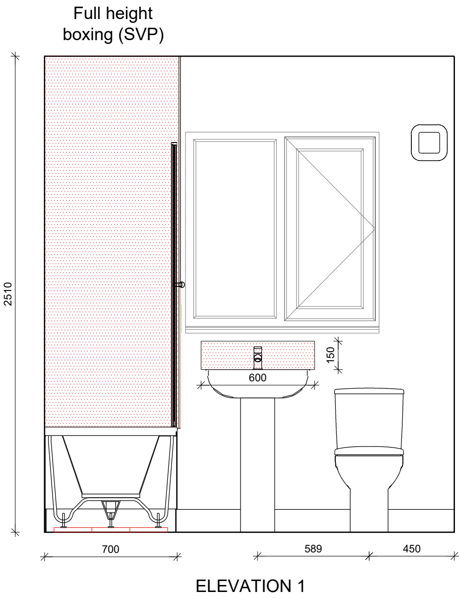
BATHROOM ELEVATIONS CARDINHAM (AS)
