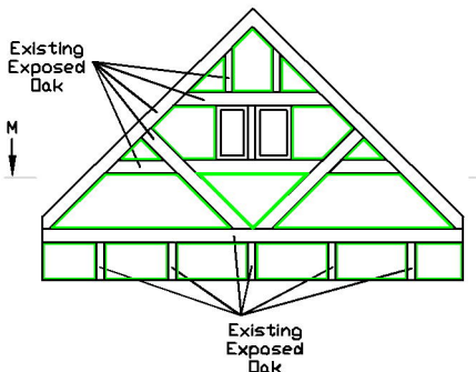
Proposed Elevation 5
