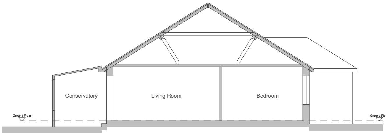
WEST SECTION/ELEVATION 1:100
