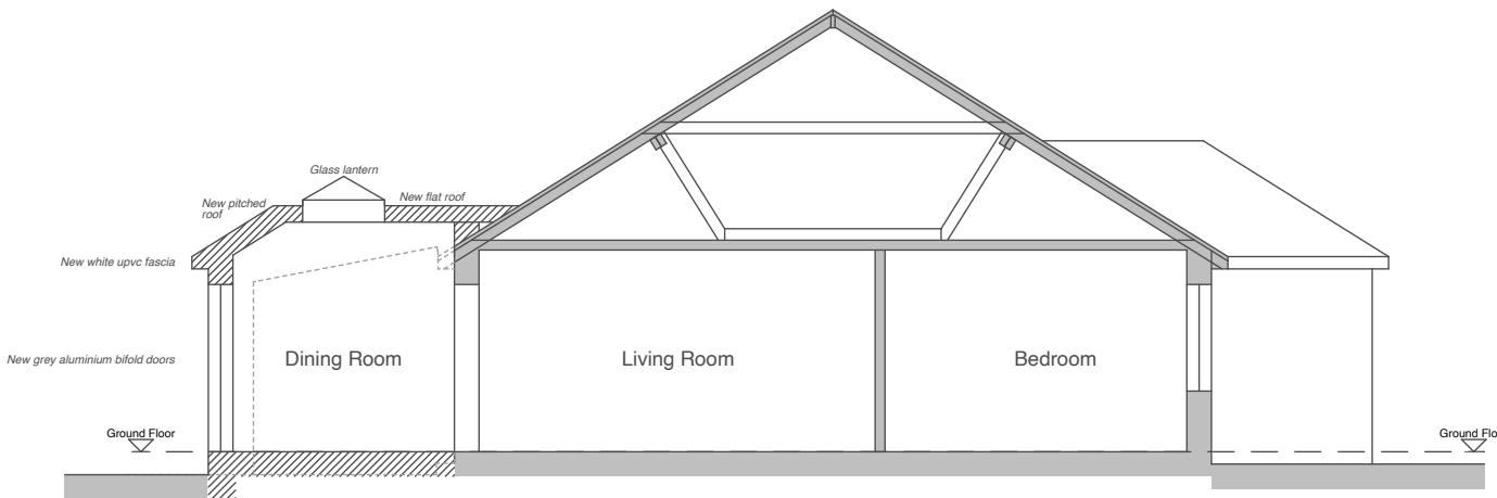
WEST SECTION/ELEVATION 1:100
