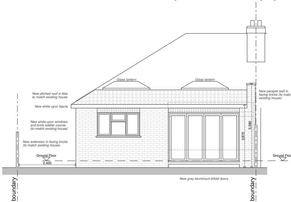
NORTH ELEVATION 1:100
